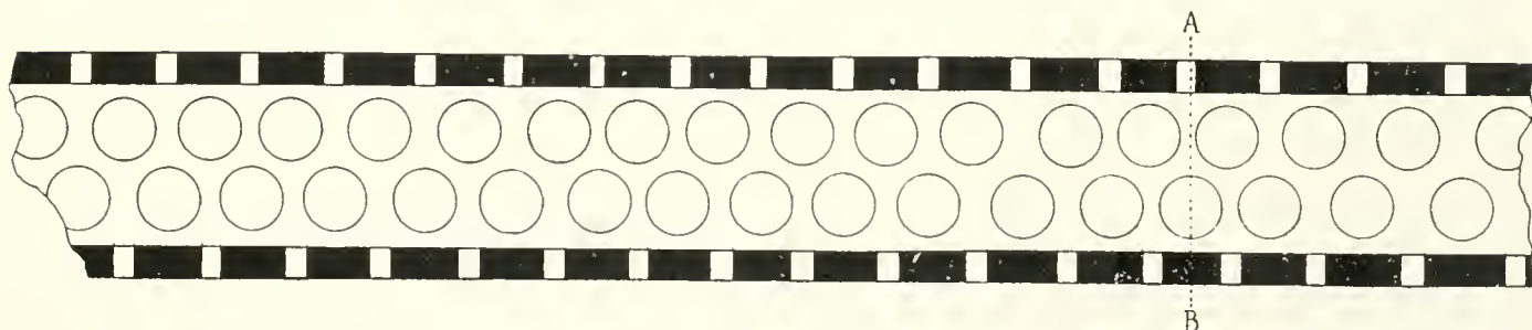
Fig. 1. Plan of the kiln. Scale \frac{1}{80} .
